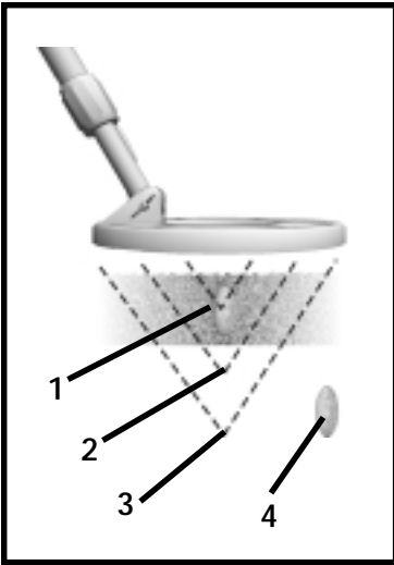
Figure 7. Search coil detection pattern and the effects of sweep, speed, trash rejection and ground mineralization.
